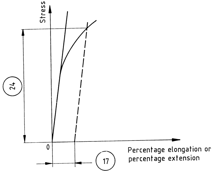
Figure 3 — Proof strength, non-proportional extension ( R_p )
