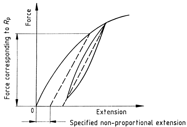
Figure 6 — Proof strength, non-proportional extension ( R_p ) (see 12.1)
