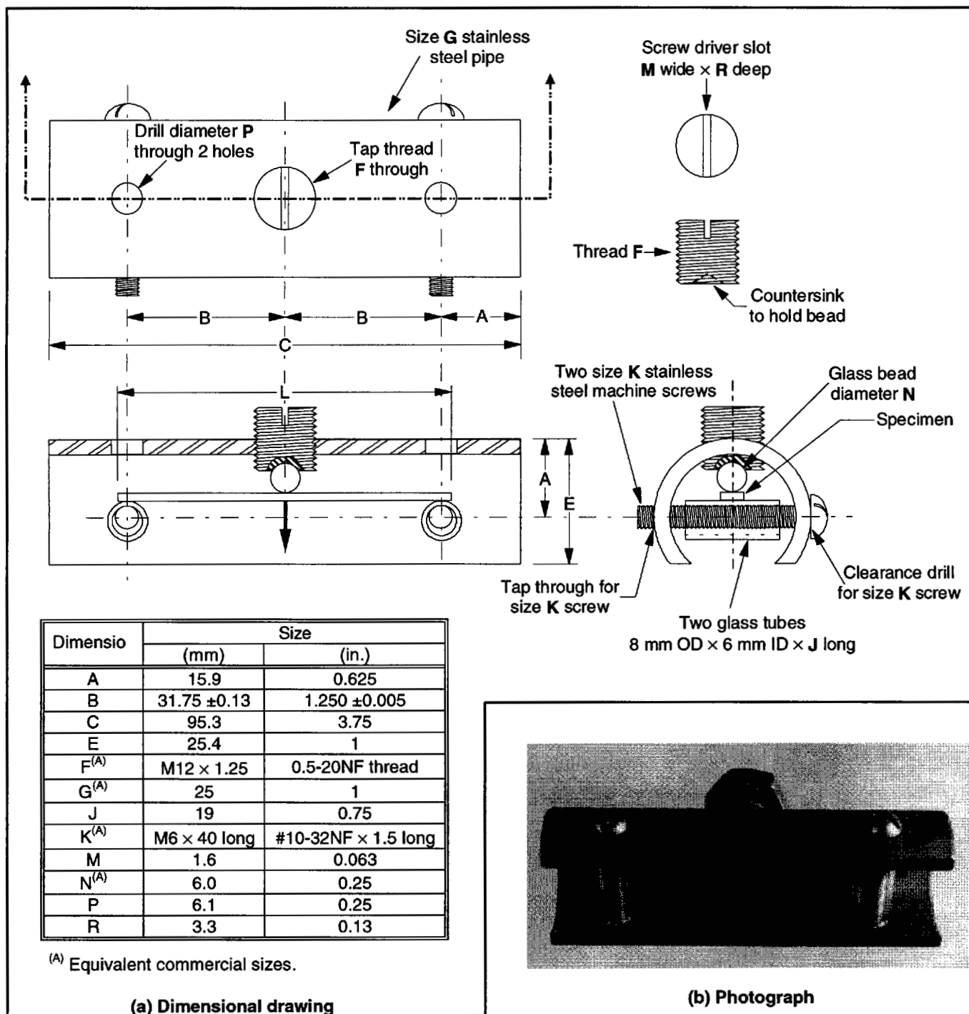
Figure 8 Typical stressing fixture for bent-beam test specimen
