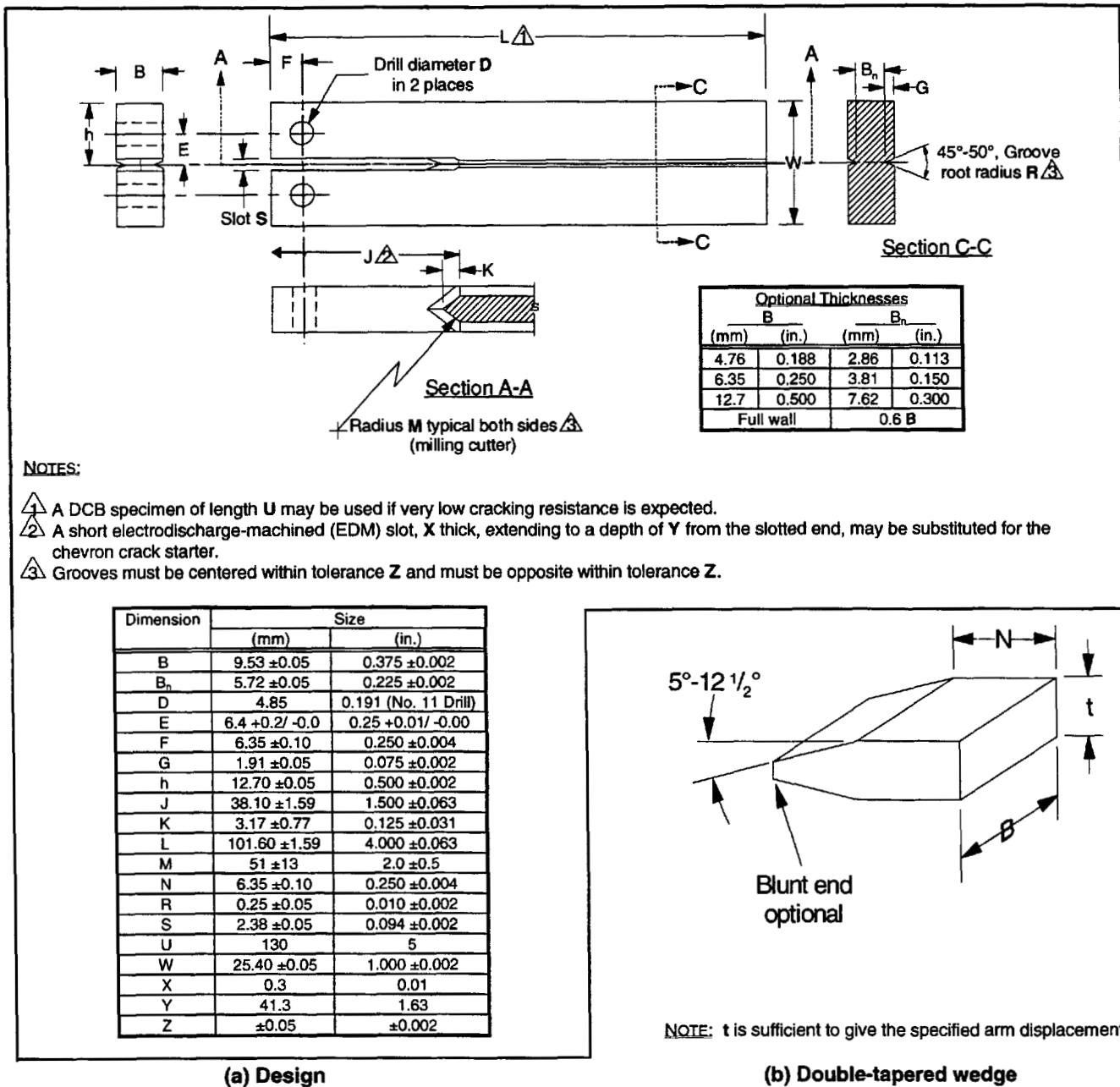
Figure 10 DCB Specimen
