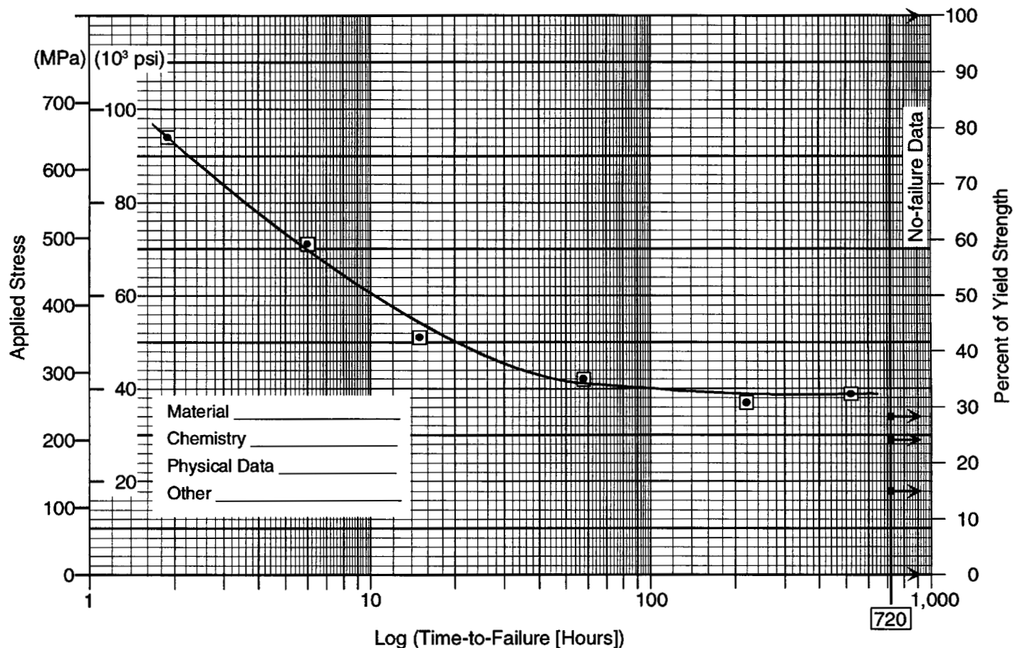
Figure 6 Applied Stress vs. Log (Time-to-Failure)
