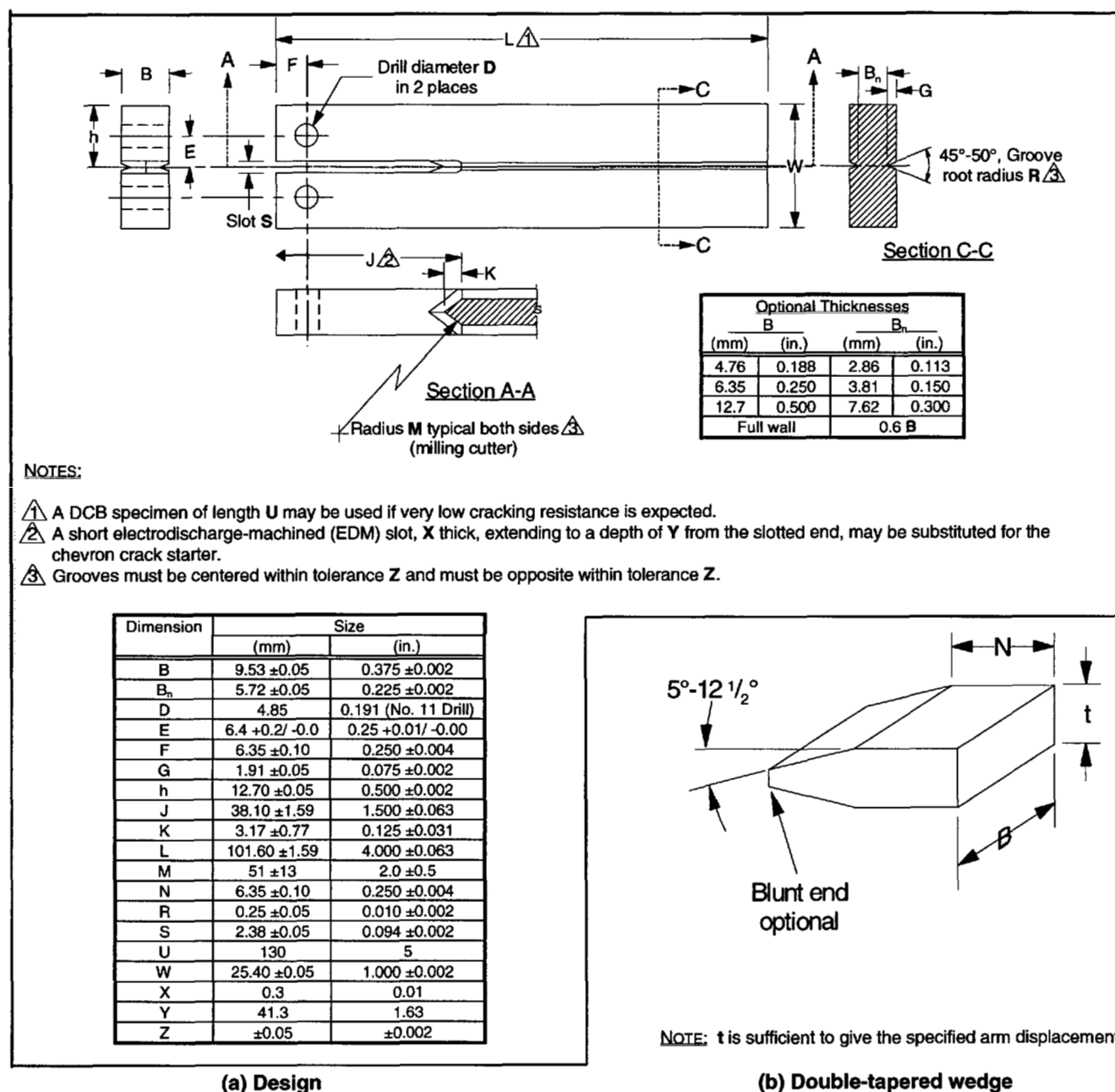
Figure 10 DCB Specimen
